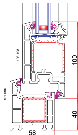
Detalle Umbral
